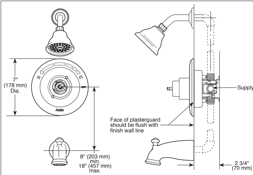
RP41589▲ Touch-Clean® Showerhead 2.0 GPM
