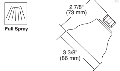
RP54752▲ H 2 O Showerhead 1.5 GPM
