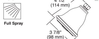
RP54752▲ H 2 O Showerhead 1.5 GPM
